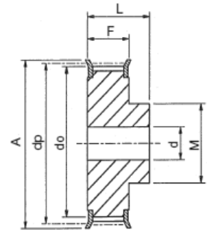
Type 1F Material: Steel
