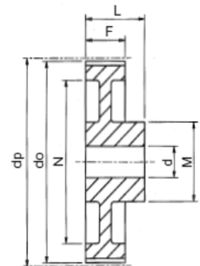
Type 2 Material: Cast Iron
