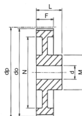
Type 2 (Aluminium)
