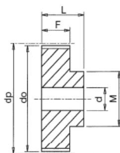
Type 1 (Aluminium)
